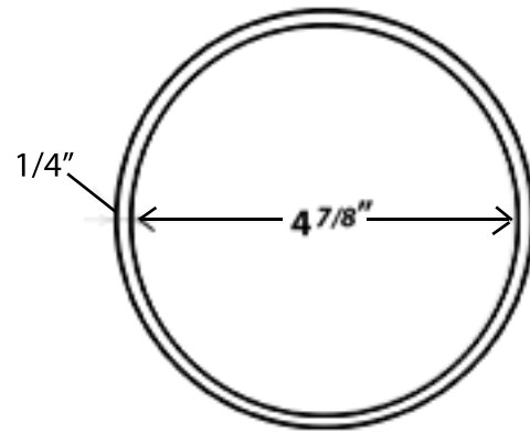
Cross Section of Sleeve
