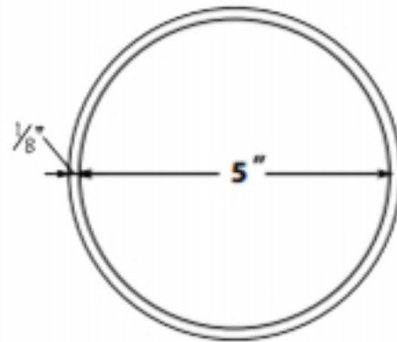
Cross Section of Sleeve
